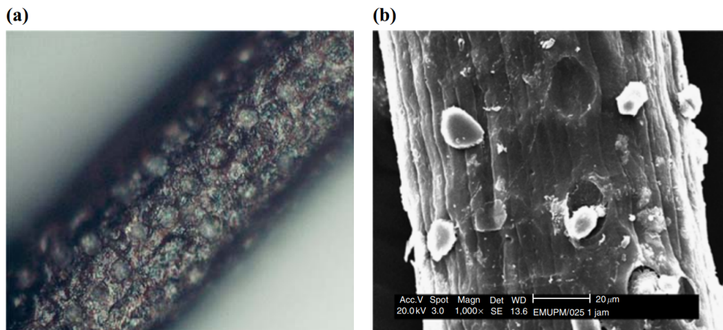
Figure 2. Natural fibre (sugar palm) anatomy in (a) Optical camera; (b) SEM micrograph. Creative Common CC BY license [23]
